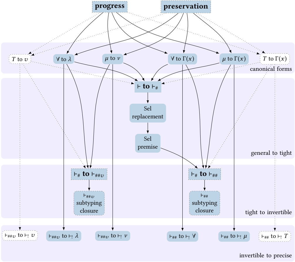
Fig. 9. Dependencies between main lemmas in the proof. Gray nodes denote existing lemmas. White nodes denote lemmas that would need to be added if DOT were extended with a new type T and a new value v . Dotted lines correspond to lemmas that will need to be added or modified for the extension.
